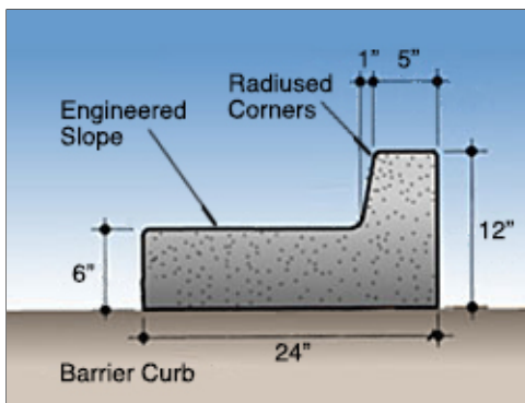
Standard Curb
