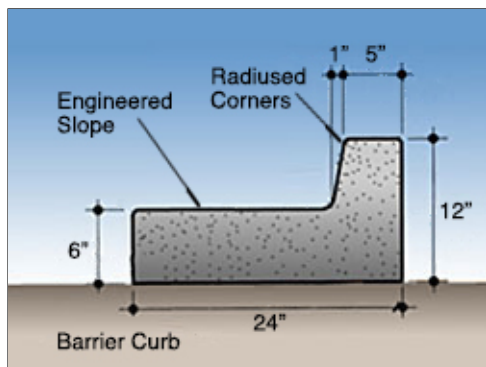
Standard Curb
